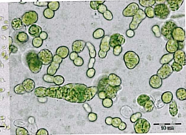
Heterococcus sp.
