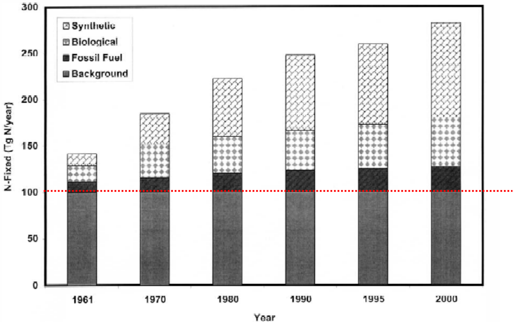
Figure 1. An estimate of total, global N fixation for 1961–2000 (adapted from Mosier et al., 2001 and Galloway et al., 1995).
